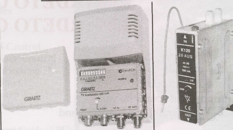
Graetz MD11P modulator produces VSB grade signals suitable for most transmission applications (left) but requiring a power "boost." K120 series amplifier (right) does just that, to 120 dBuV. Graphics courtesy Lacey's.TV.
