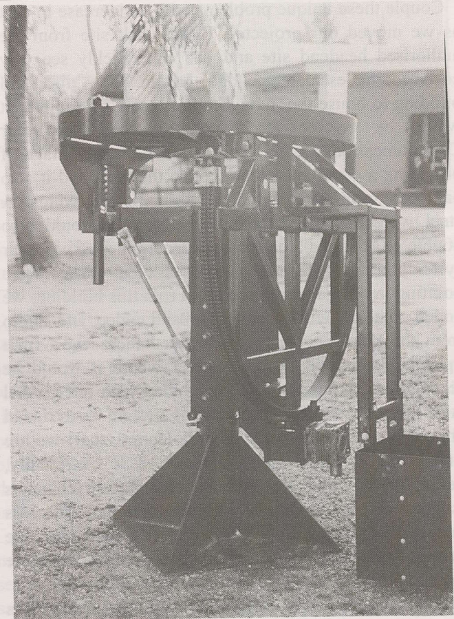
In short order the T24 "pieces" begin to add up to some very significant weight. Here, the tower-topping dish support and rotational system.
