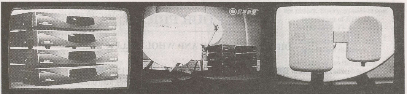
SPACE Systems IRD units (left) as displayed on barker channel promotional tape; "Acer" satellite dishes (offset-left, prime focus right); Offset LNB mounted on offset dish for North American reception of SPACE Ku feed on Galaxy 4 (99W) with dish system originally installed for DirectTV DBS (101W).
