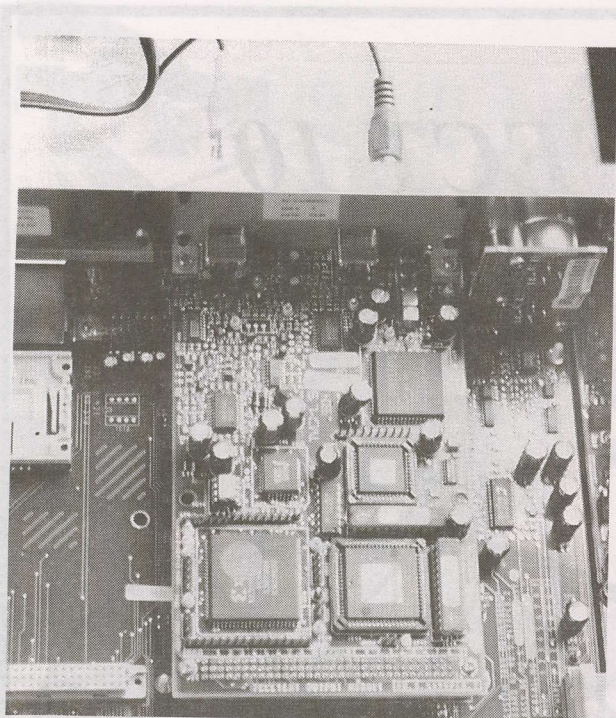
Did its' job. Special DMV created plug-in board (top, centre) mounted inside DMV 3000 receiver produced MediaNet within VBI. But a consumer grade decoder that followed left us high and dry.
