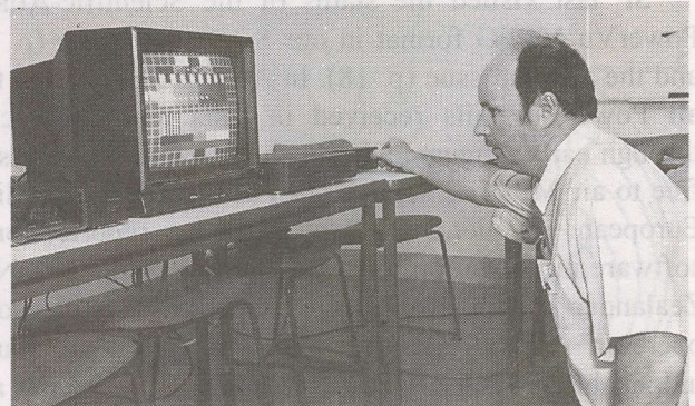
Barry Ward (Auckland) has built a satellite spectrum analyser using commonly available (Dick Smith) parts and a 'junker' oscilloscope. He will explain how he did this and give assistance to others in duplicating his "low cost analyser" (as little as $300) during SPRSCS '97.
