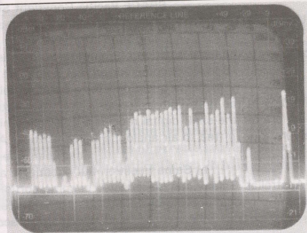
Spectral display showing 39 cable TV carriers from 55.25 MHz (left hand side) to 447.25 (right).
