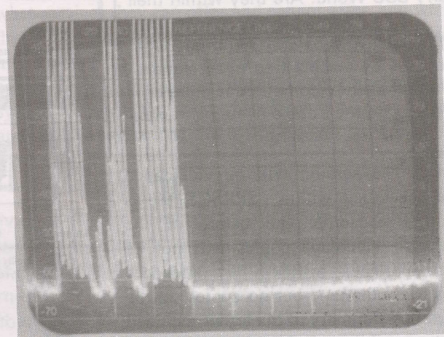
How far "down?" Top two displays are in 10 dB per graticule division. Here, 15 carriers remaining after the filter is installed are displayed at 2 dB per division. Carriers in cut-off region are "down" more than 50 dB; more than enough to eliminate service to TV sets above the cut-off frequency.
