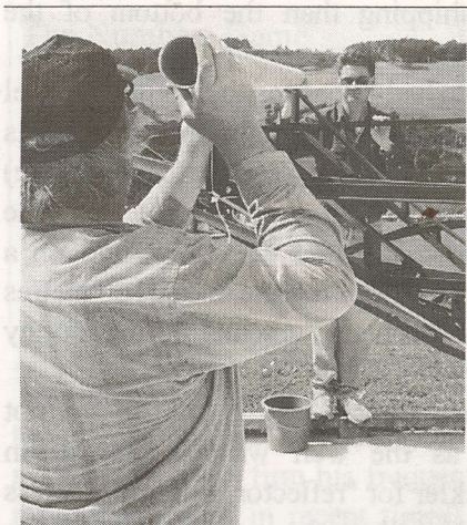
Truing the ribs, using the taunt rib strings as a reference, with (PVC) straight edge.
