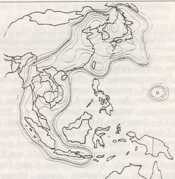
Palapa C1 Ku band coverage is Asia only with 50 dBw at centres (additional contours down in 1dB steps)
