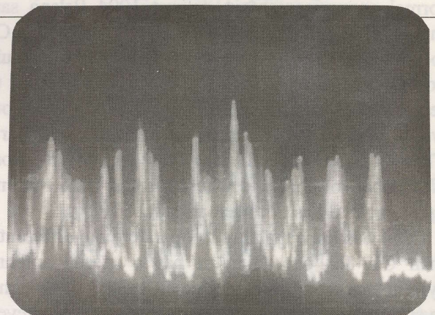
On spectrum analyser, these 'carriers' appear as discrete signals; in fact, each 'blip' (carrier) may contain several hundred discrete narrowband channels!
