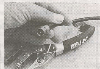
Finished Connector
