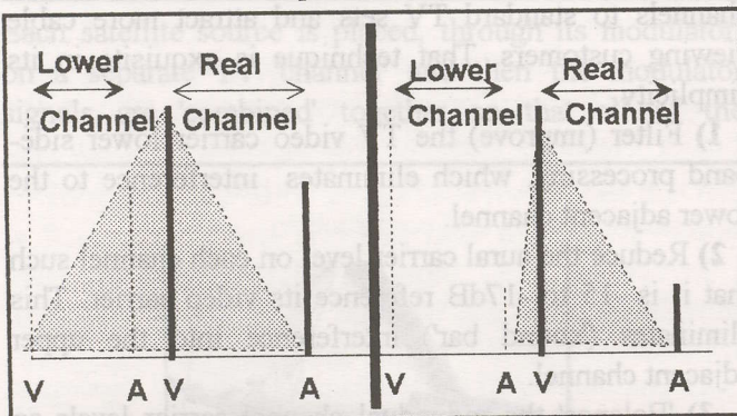
Double sideband (DSB) modulator (left) spreads video energy down into lower adjacent channel; Vestigial sideband (VSB) modulator (right) keeps energy inside single channel, eliminates lower channel interference.
