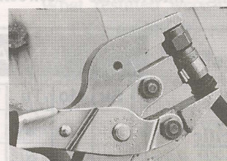
Torque Ring Into Fitting
