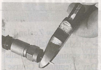
Trim Centre Conductor
