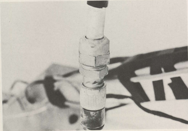
SPLICE of RF line — transition from hardline (top) to flexible cable that allows rotation of feed plus LNA 'begs' for moisture entry.
