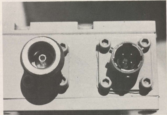
TWO POINTS OF ENTRY — in typical LNA package. RF connector (type 'N') is on left ; powering plug is on right. Powering connections require great care because the wire-end of fitting cannot handle wire diameters over #20/22 safely.
