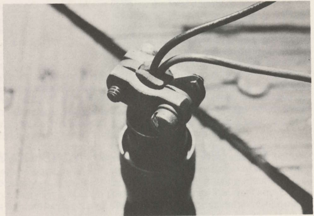
UNPROTECTED — DC powering plug is fitted with weather protection sealing grommet. Unfortunately the plug faces 'upwards' into the sky and rain can puddle inside of fitting.
