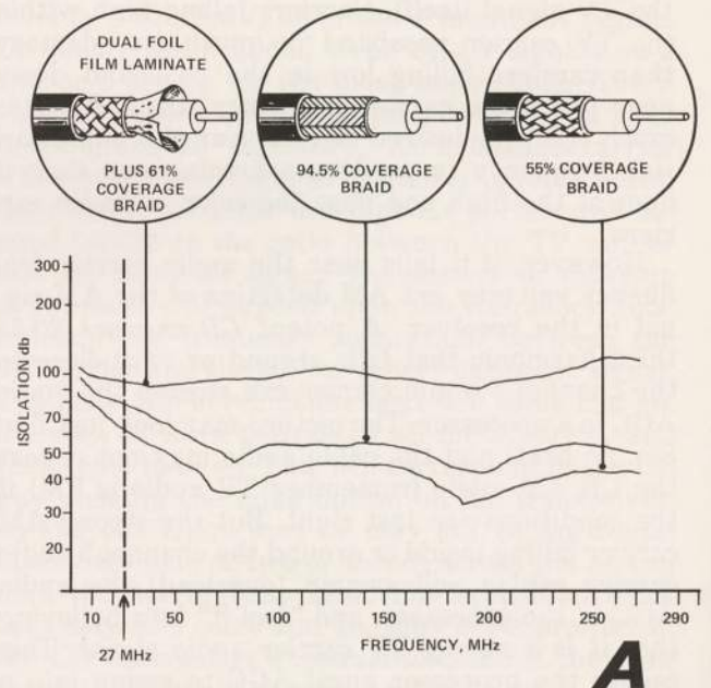
BELDEN SEED PERFORMANCE CURVES DETAIL SHIELD EFFECTIVENESS COMPARISONS
