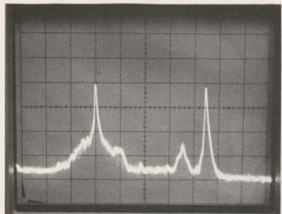
PHOTO FOUR—And now the vertical scale is switched to 10 dB per division and 30 kHz i.f. bandwidth. The difference between photos one and four? In "one" we are looking at the "tip-top" of the signal carriers while with photo "four" we have a "depth of field" allowing us to look down the side of the carrier clear to the bottom of the signal voltage and to the floor or base noise floor of the system (in "this case" approximately 36 dB signal to noise ratio at 10 dB per division).
