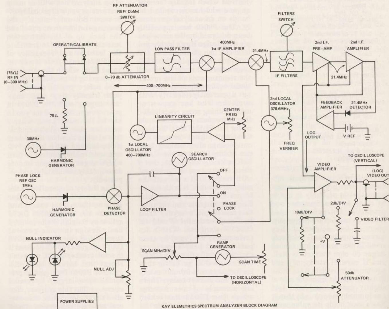
KAY ELEMETRICS SPECTRUM ANALYZER BLOCK DIAGRAM
