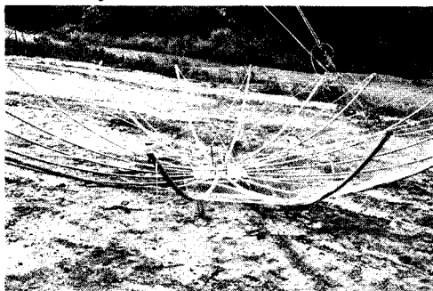
Mesh screening is installed from top to bottom, starting at center working out.
