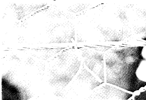
Where screen crosses tension wire, use lashing wire to clamp into position.
