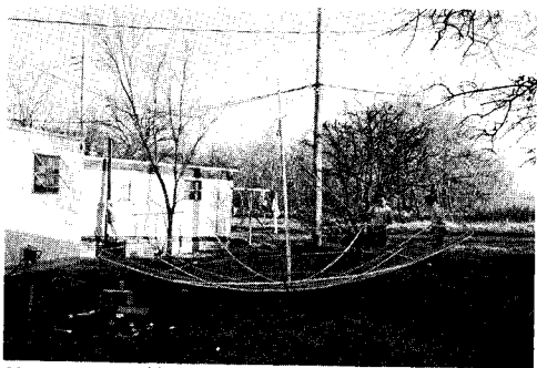
24' all aluminum super structure parabolic with center mounted feed.
