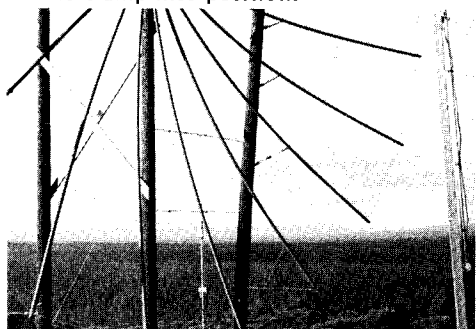
Oregon 40' construction utilizes poles as back supports on struts.
