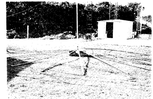
All struts in place, and tension wires strung through eyebolts, ready for "come-along" pull.
