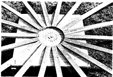
18 struts are laid out per text on plywood backplate.
