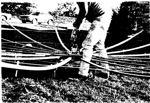
With struts under tension, steel front plate is installed over ply backplate (Diagram 12).
