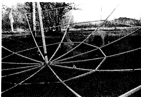
Screen mesh is anchored to struts and braces.
